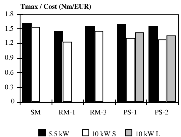
Figure 8. Pull-out torque per the cost of active materials. Solid (S) and laminated (L) pole shoes.
