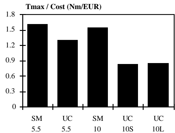
Figure 18. Pull-out torque per the cost of active materials. Solid (S) and laminated (L) rotor core.
