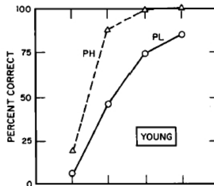
Figure 3.1: Example of SPIN test results.
