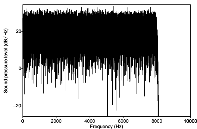
Figure 4.3: Filtered white noise used as a masker in this study
