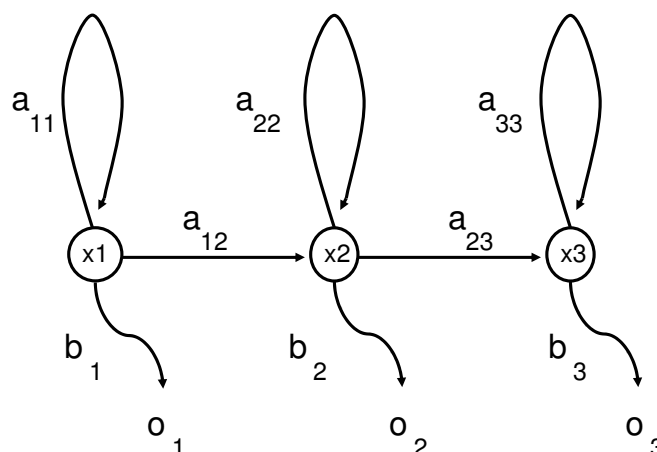
Figure 2.3: A three state left-to-right HMM with states x_x , transition probabilities a_{xx} , output probabilities b_x , and observations o_x
