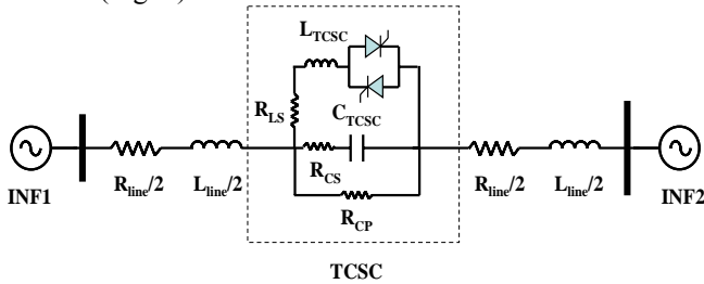
Fig. 3. Structure of the power system modeled in the studies
