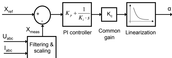
Fig. 4. Structure of fundamental reactance control
