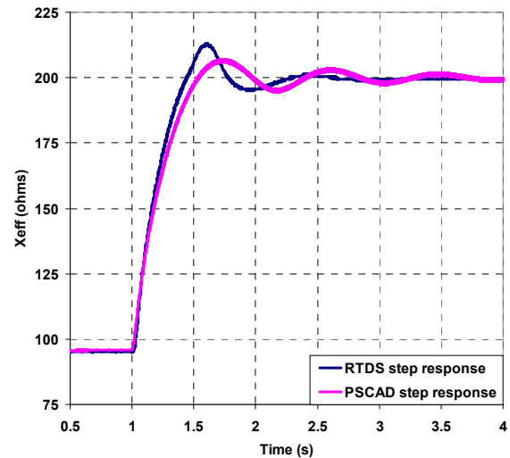
Fig. 6. Step response of closed-loop fundamental reactance control in PSCAD and RTDS
