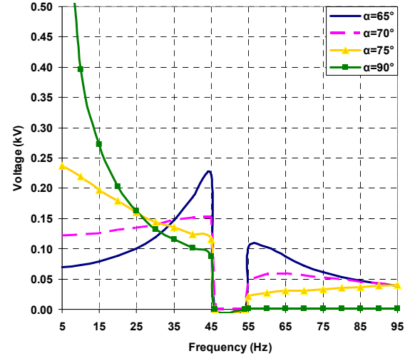
Fig. 10. Induced voltage components with different firing angles of TCSC
