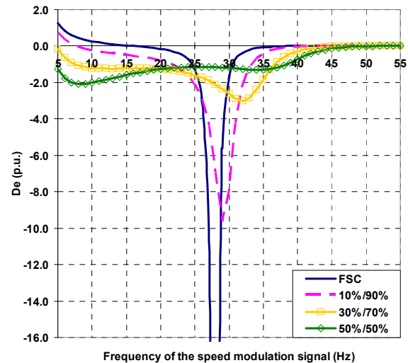
Fig. 8. Damping coefficient with different proportion of TCSC to FSC [5]
