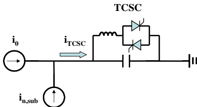
Fig. 9. Test system for illustrating the sub- and supersynchronous response of TCSC
