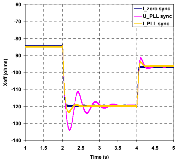
Fig. 7. Step response of different synchronization methods
