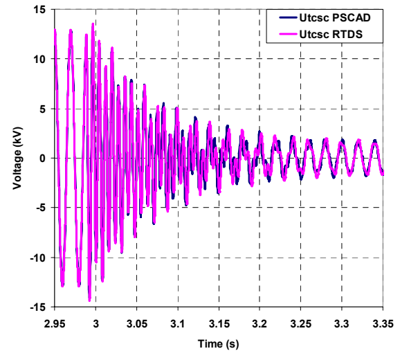
Fig. 5. Mode switching from blocking mode to bypass mode in PSCAD and RTDS
