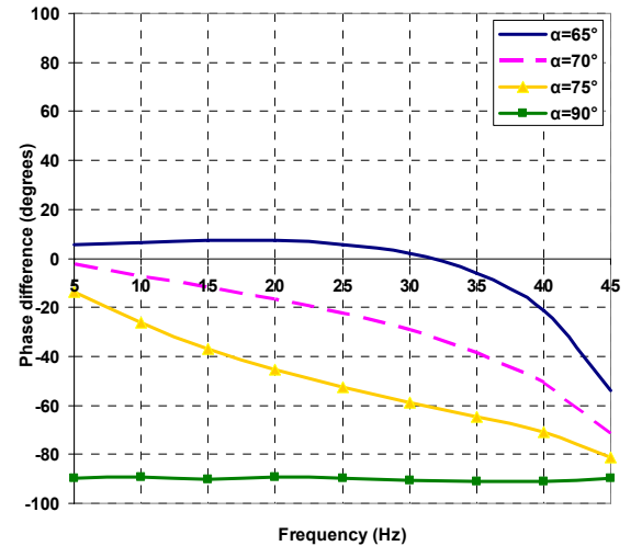
Fig. 11. Phase relation between injected current components and induced voltage components
