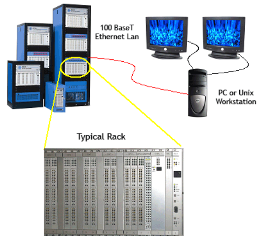
Fig. 2. Typical RTDS configuration [4]
