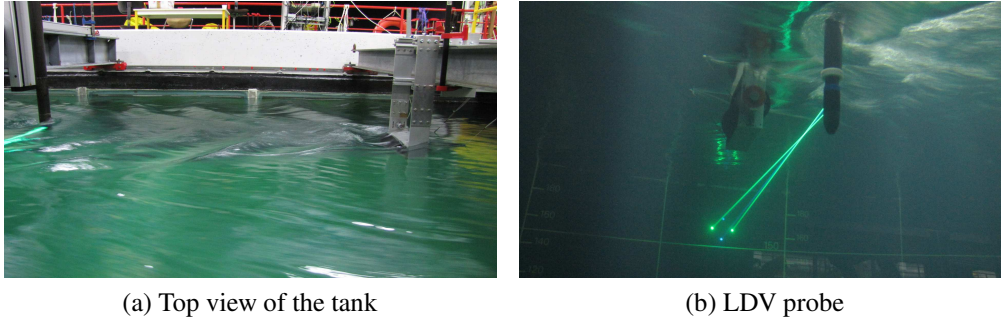
Figure 7: Experimental facility at IFREMER, France
