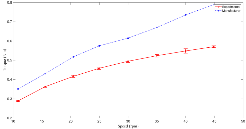
Figure 6: Relation of torque and speed of a dashpot with viscosity of 250 cst
