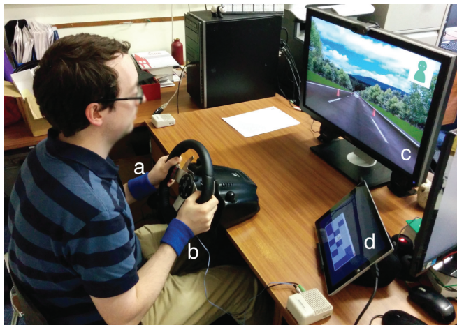
Figure 1. The setup of the experiment with the tactile wristbands (a, b), the driving simulator (c) and the tablet (d)
