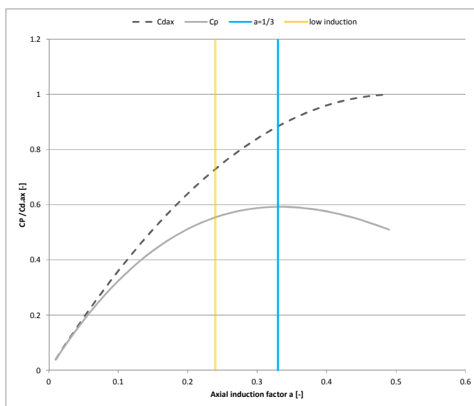
Figure 1. Power and axial force coefficient as function of axial induction factor. Lines for maximum power coefficient ( a=1/3 ) and low induction are indicated
