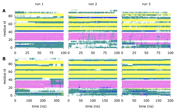
FIG. 4: Secondary structure per residue of wild-type Rsn-2 at (A) air-water and (B) oil-water interfaces as a function of time (magenta \alpha -helix, blue 3/10 helix, yellow \beta -sheet, green turn).
