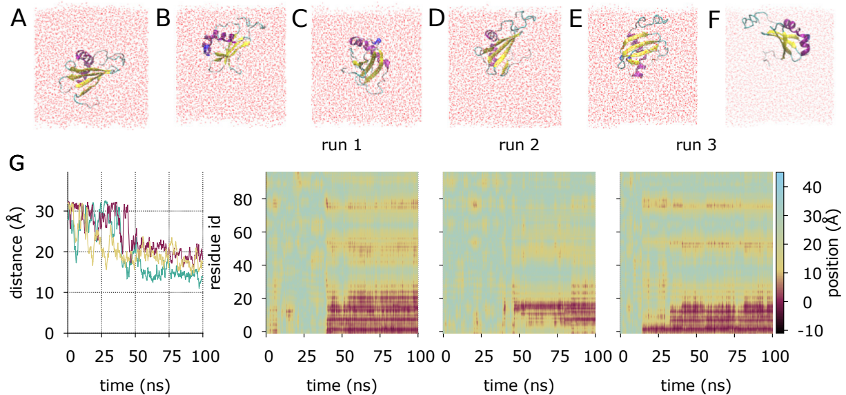
FIG. 2: Adsorption of wild type Rsn-2 at an air-water interface. (A-F) Snapshots of Rsn-2 adsorption observed in the first simulation run at times (left to right) 0, 5, 15, 38, 55 and 100 ns. (G) Distance of the protein centre of mass from the interface and residue-interface separations as a function of time. Cyan, red, and yellow lines denote first, second, and third runs respectively.
