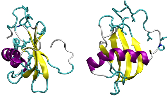
FIG. 1: NMR solution structure of Rsn-2 (PDB: 2WGO, first frame) . Left shows view parallel to \alpha -helix axis, highlighting the side-chains of the hydrophobic core. Right view normal to \alpha -helix axis, showing the hydrophobic side-chains on the N-terminal tail.
