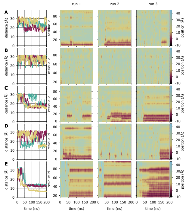
FIG. 7: Distance of the centre of mass from the interface and residue-interface separations for Rsn-2 mutants: (A) \Delta L1-L3, (B) \Delta L1-P15, (C) \Delta Y96 and (D) \Delta D89-Y96 at the air-water interface, and (E) \Delta L1-P15 at the oil-water interface. For the distance, cyan, red, and yellow lines denote first, second, and third runs respectively.
