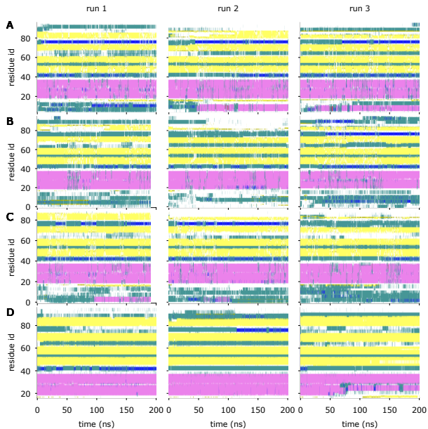
FIG. 8: Secondary structure per residue as a function of time for the Rsn-2 mutants: (A) \Delta L1-L3, (B) \Delta Y96 and (C) \Delta D89-Y96 at the air-water interface, and (D) \Delta L1-P15 at the oil-water interface. We excluded \Delta L1-P15 Rsn-2 at an air-water interface from the figure, since it does not adsorb in any of the considered runs and it is stable in the bulk.
