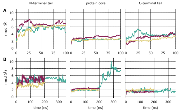
FIG. 5: Backbone root mean square displacement from the initial conformation of wild-type Rsn-2 at (A) air-water and (B) oil-water interfaces for the N-terminal tail (from the tag to residue id 15), the structured core (residues id 16-88) and the C-terminal tail (from residue id 89).
