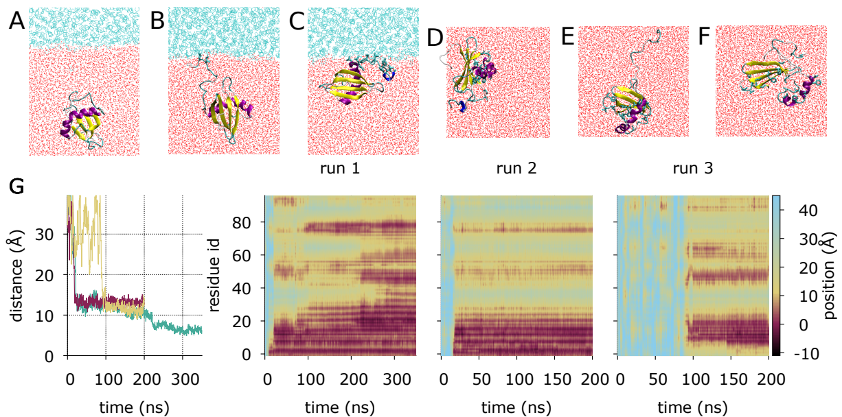
FIG. 3: Adsorption of wild type Rsn-2 at a cyclohexane-water interface. (A-F) Snapshots of Rsn-2 adsorption observed in the first simulation run corresponding, from left to right, to times 0, 12, 24 (side view and top view), 131 and 263 ns. (G) Distance of the protein centre of mass from the interface and residue-interface separations as a function of time. Cyan, red, and yellow lines denote first, second, and third runs respectively.
