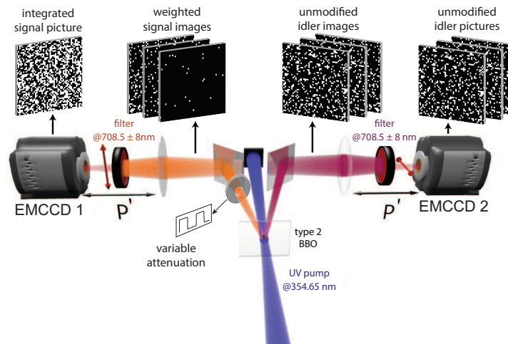
FIG. 1: Experimental setup used to record the ghost signal and the reference idler images. The red arrows represent the polarisation directions of the signal and idler beams. The variable attenuation, made with a liquid crystal variable retarder and a polariser, is adjusted accordingly.
