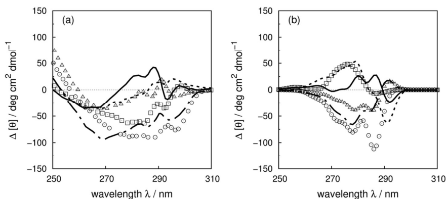
Figure 11. Difference spectra (wild-type minus the mutants) of human carbonic anhydrase II ((a): experiment; (b): calculation); \Delta W5F (solid line), \Delta W16F (square), \Delta W97C (circle), \Delta W123C (triangle), \Delta W209F (dotted line) and \Delta W245C (dot-dashed line).
