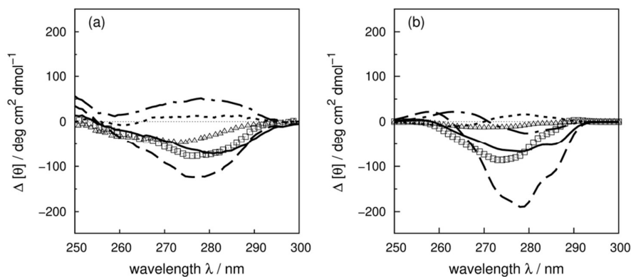
Figure 10. Difference spectra (wild-type minus the mutants) of RNase A ((a): experiment; (b): calculation). \Delta\text{Y}25\text{F} (solid line), \Delta\text{Y}73\text{F} (dashed line), \Delta\text{Y}76\text{F} (dotted line), \Delta\text{Y}92\text{F} (triangle), \Delta\text{Y}97\text{F} (dot-dashed line) and \Delta\text{Y}115\text{F} (square).
