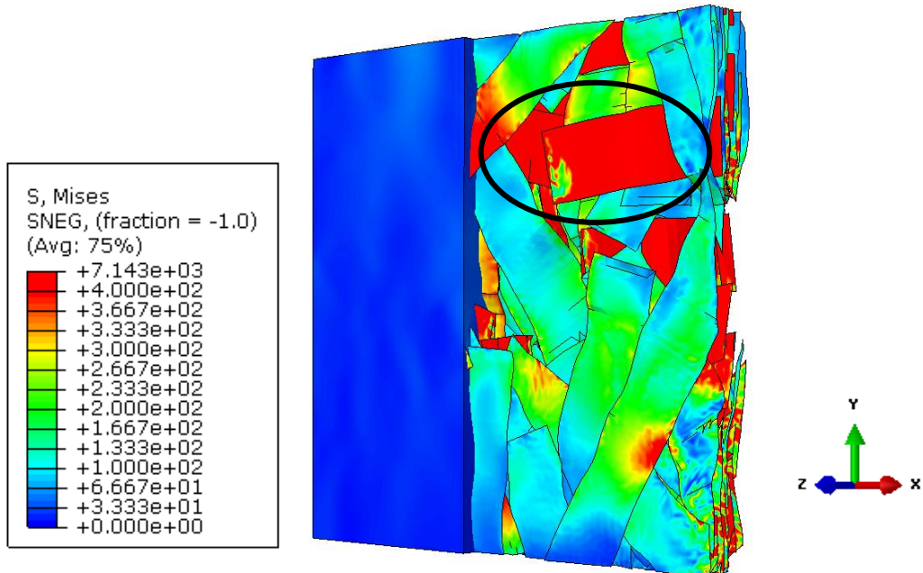
Figure 10: von Mises plot for a 10% Vf, 38x38x3mm RVE at a global applied tensile strain of 0.8% in the x-direction (prior to coupon failure). Plot scaled between 0-400MPa to highlight stress in fibre. Section of resin removed to display internal fibres. Black circle highlights highly stressed fibre along loading direction.
