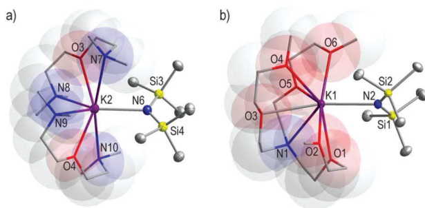
Fig. 6 (a) Molecular structure of [\text{KHMDS}(\text{TMDAE})_2] 10 , showing one of the two crystallographically independent molecules within the asymmetric unit. (b) Molecular structure of [\text{KHMDS}(\text{TMEEA})] 11 . Hydrogen atoms are omitted for simplicity. Displacement ellipsoids are displayed at 35% probability. The TMDAE and TMEEA ligands are pictured in 10 and 11 as capped sticks with translucent space-filling van der Waals surfaces for a probe of 1.5 Å radius. Selected bond distances (Å) and angles (°): for 10 , K2–N6 2.794(3), K2–O3 2.814(2), K2–O4 2.824(2), K2–N9 2.960(3), K2...N10 3.559(3), K2–N8 2.975(3), K2...N7 3.337(3), N6–K2–O3 111.44(8), N6–K2–O4 106.42(9), O3–K2–O4 141.91(8), N6–K2–N9 132.63(8), O3–K2–N9 95.50(9), O4–K2–N9 60.13(9), N6–K2–N8 134.58(9), O3–K2–N8 59.22(8), O4–K2–N8 90.93(9), N9–K2–N8 92.54(9), N6–K2–N7 83.46(9), O3–K2–N7 55.33(8), O4–K2–N7 135.52(8), N9–K2–N7 81.01(9), N8–K2–N7 113.00(9), N6–K2–N10 83.97(8), N10–K2–N7 166.99(8); for 11 , K1–O1 2.7613(8), K1–N2 2.7889(9), K1–O6 2.8131(8), K1–O4 2.8736(8), K1–O5 2.9078(8), K1–O3 2.9652(8), K1–N1 3.1364(9), K1...O2 3.3145(10), O1–K1–N2 80.00(3), O1–K1–O6 150.12(3), N2–K1–O6 83.93(3), O1–K1–O4 137.21(3), N2–K1–O4 121.03(3), O6–K1–O4 72.63(2), O1–K1–O5 111.53(2), N2–K1–O5 122.61(2), O6–K1–O5 57.96(2), O4–K1–O5 88.90(2), O1–K1–O3 90.45(2), N2–K1–O3 161.50(2), O6–K1–O3 111.11(2), O4–K1–O3 57.56(2), O5–K1–O3 75.61(2), O1–K1–N1 57.01(2), N2–K1–N1 126.60(2), O6–K1–N1 117.35(2), O4–K1–N1 112.19(2), O5–K1–N1 59.71(2), O3–K1–N1 57.04(2), O1–K1–O2 56.12(2), N2–K1–O2 85.08(3), O6–K1–O2 147.03(2), O4–K1–O2 86.86(2), O5–K1–O2 149.24(2), O3–K1–O2 76.45(2), N1–K1–O2 94.02(2).
