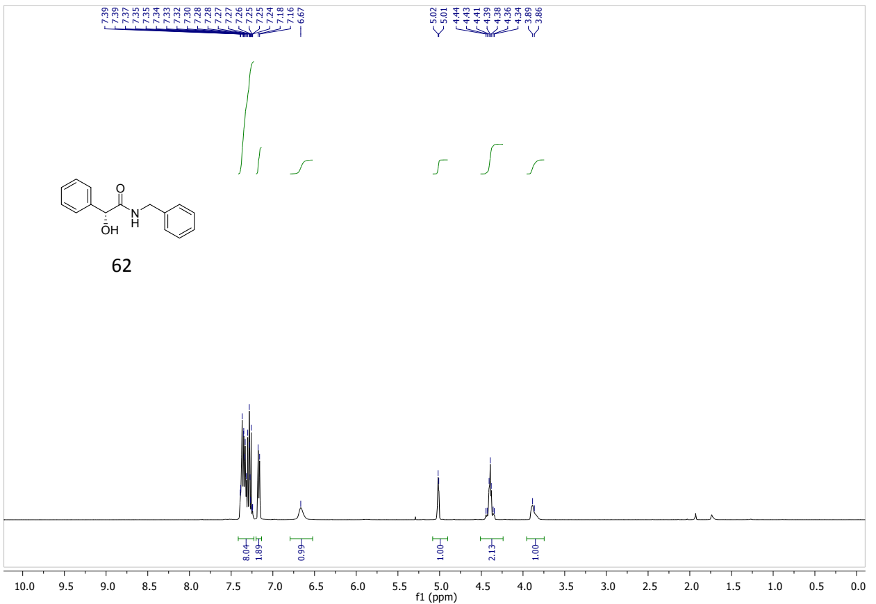
(R)-N-benzyl-2-hydroxy-2-phenylacetamide (62)
