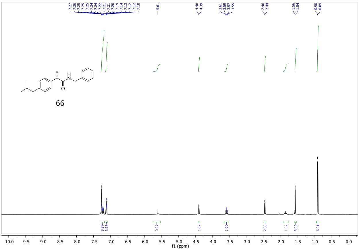
(S)-N-benzyl-2-(4-isobutylphenyl)propanamide (66)
