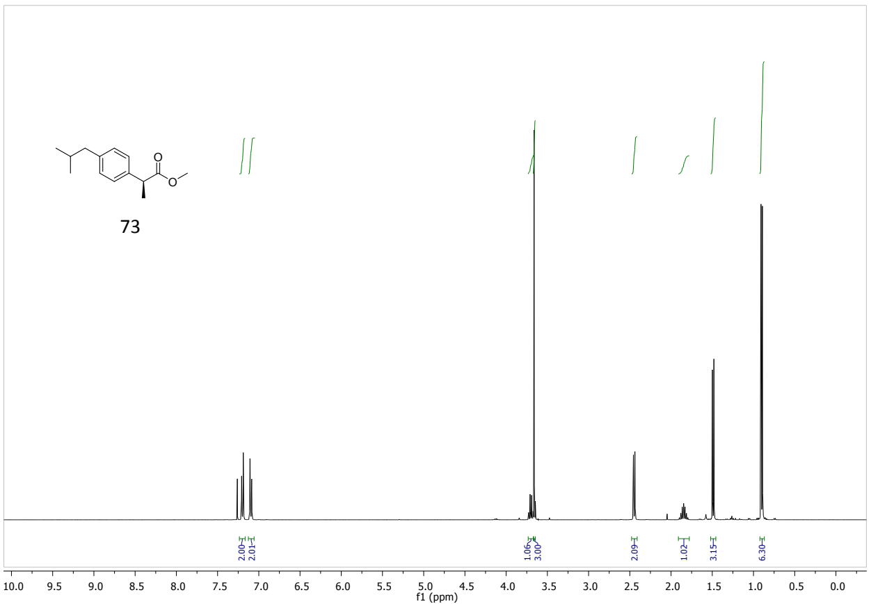
Methyl (S)-2-(4-isobutylphenyl)propanoate (73).
