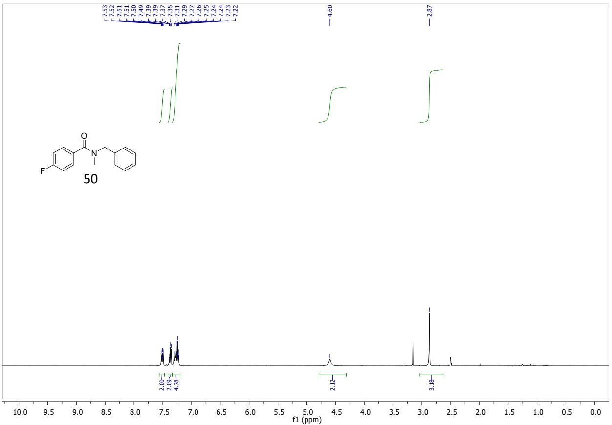
N-benzyl-4-fluoro-N-methylbenzamide (50)
