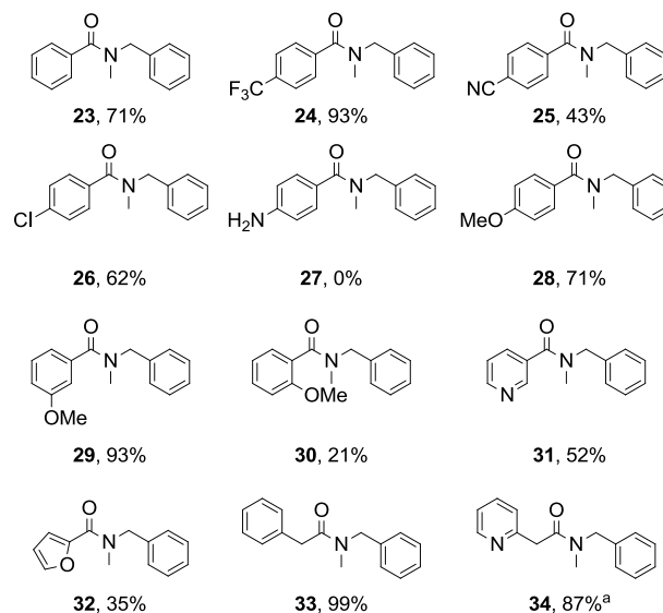
Scheme 3. Investigating the scope of the ester component. a Synthesised from the corresponding ethyl ester starting material.
