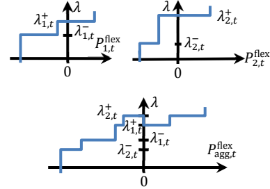
Fig. 4 Generator (1), load (2) and (3, bottom) aggregated bid functions.
