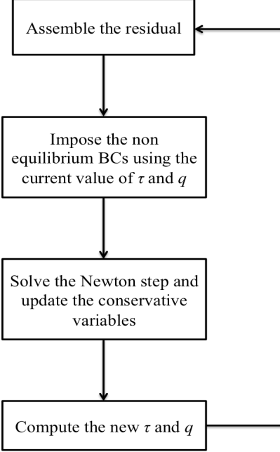
Figure 1. Algorithm for the imposition of the velocity slip and temperature jump using CGFEM.
