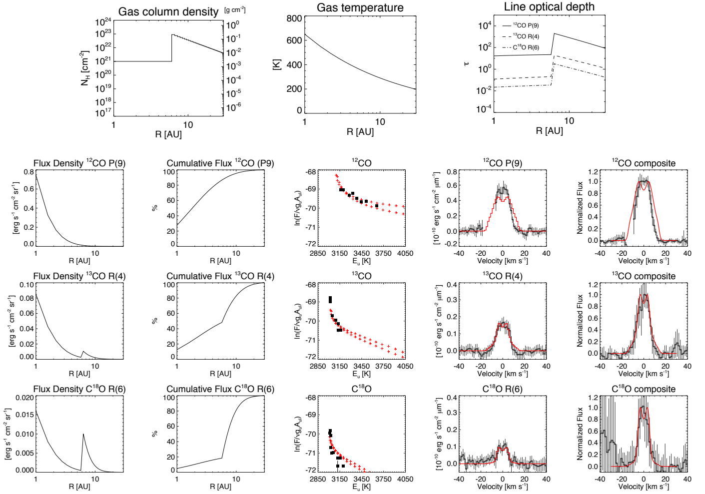
Fig. C.2. Surface density, temperature, CO optical depth, flux density, cumulative line flux, rotational diagrams, line profiles of the 12 CO P(9), 13 CO P(4), and C 18 O R(6) emission, for the best model in the grid when \alpha_{N_{H\text{inner}}} \leq +1.0 . Model is in red observations are in black. Observed line profiles are displayed in flux units after continuum subtraction with 3 \sigma error bars. The two branches seen in the rotational diagram correspond to the R and P branches of CO ro-vibrational emission. The right-most panels compare the normalized theoretical line profiles with the observed composite line profile of each CO isotopologue with a 1 \sigma error bar.
