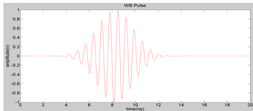
Fig. 2. The transmitted Gaussian pulse with: f_L = 1.19 GHz; f_H = 1.65 GHz.
