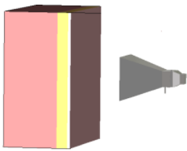
Fig. 1. The tissue model is placed 60 mm apart from the DRH antenna.
