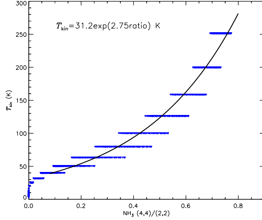
Figure A6. The \text{NH}_3 (4, 4)/(2, 2) line ratios and the kinetic temperatures from RADEX models. At each temperature, we took the line ratios from models with \text{H}_2 densities between 10^4 and 10^5 \text{ cm}^{-3} , and column densities between 5 \times 10^{22} and 5 \times 10^{23} \text{ cm}^{-2} . The solid line is a least-square fit to the ratio- \log(T_{\text{kin}}) relation between T_{\text{kin}} = 30\text{--}300 \text{ K} .
