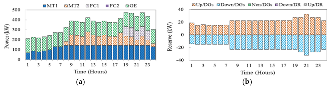
Figure 7. Hourly energy and reserves scheduling in case 2 under TOU programs (a) energy and (b) reserve.
