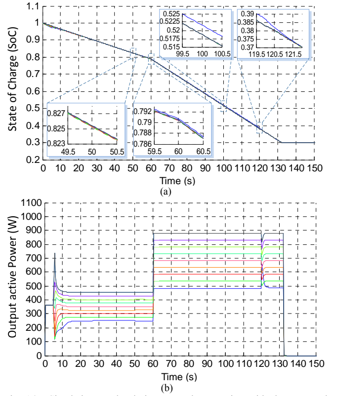
Fig. 16. Simulation results during network separation with the proposed DCA-based coordinated control. (a) SoC of ESSs. (b) Active power output of DGs.
