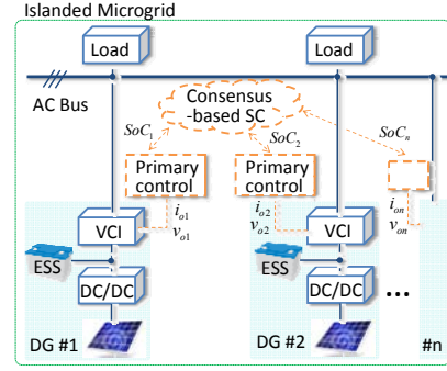
Fig. 1. PV-ESS-based AC MG case study scenario.
