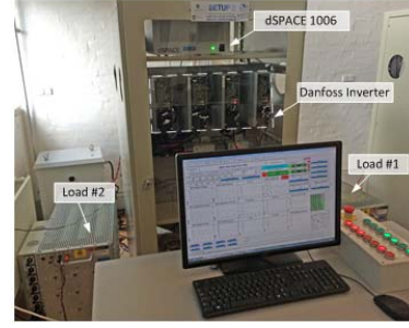
Fig. 9. Experimental setup.
