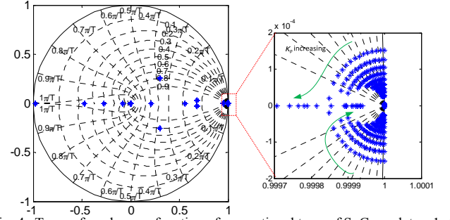
Fig. 4. Trace of modes as a function of proportional term of SoC regulator: 1 < K_p < 2000 , (cross topology).
