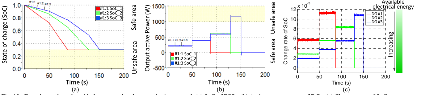
Fig. 10. Experimental results with the conventional power sharing control. (a) SoC of ESSs. (b) Active power output of DGs. (c) Change rates of SoC.
