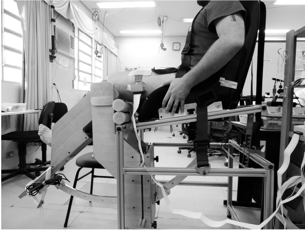
Figure 1 – Experimental setup illustrating the electrode matrix placed at vastus lateralis for sEMG recordings with the knee positioned at 45° degrees (0° = full extension) in the dynamometer.
