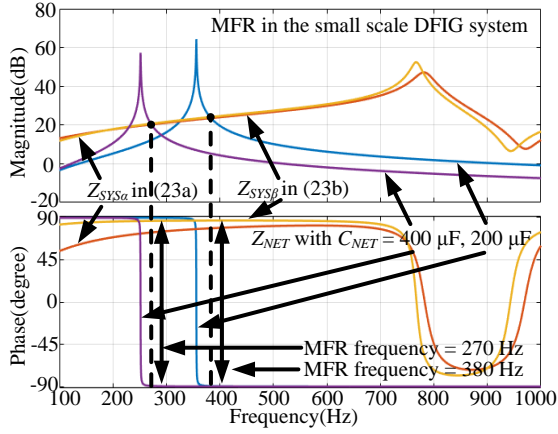
Fig. 9. Bode diagram of the 7.5 kW DFIG system impedance Z_{SYS} with fast PLL control parameters K_{ppll} = 50 , K_{ipll} = 500 , and the parallel compensated weak network with C_{NET} = 200 \mu\text{F} , 400 \mu\text{F}
