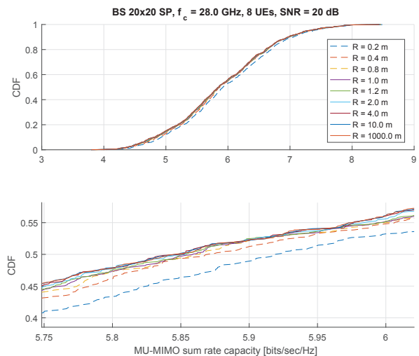
Fig. 9. CDFs of MU-MIMO sum rate capacities with different measurement distances R (top) and a zoomed in view of it (bottom).
