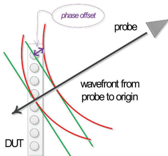
Fig. 3. Definition of phase deviation between a planar and a spherical waves across the DUT.
