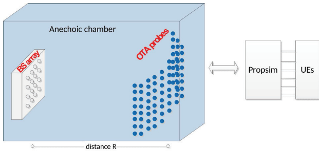
Fig. 1. Sketch of sectored MPAC setup.
