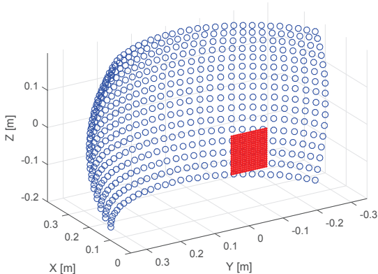
Fig. 2. The setup of probes (blue) and DUT array (red).
