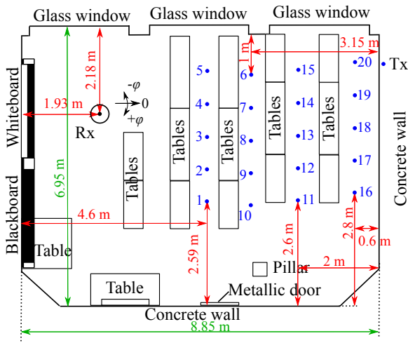
Fig. 2: Floor plan with Tx and Rx locations
