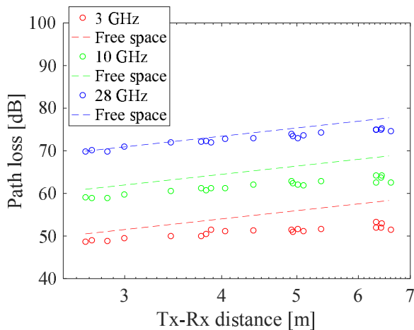
Fig. 7: Path loss comparison with free space path loss
