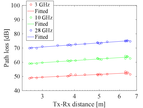
Fig. 8: Path loss model parameters fitting results
