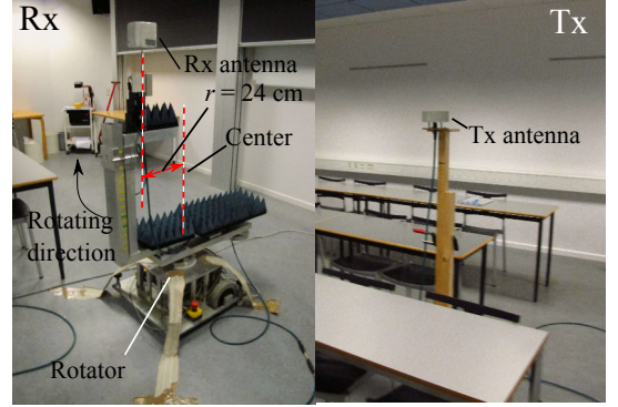
Fig. 3: Photo of the measurement
