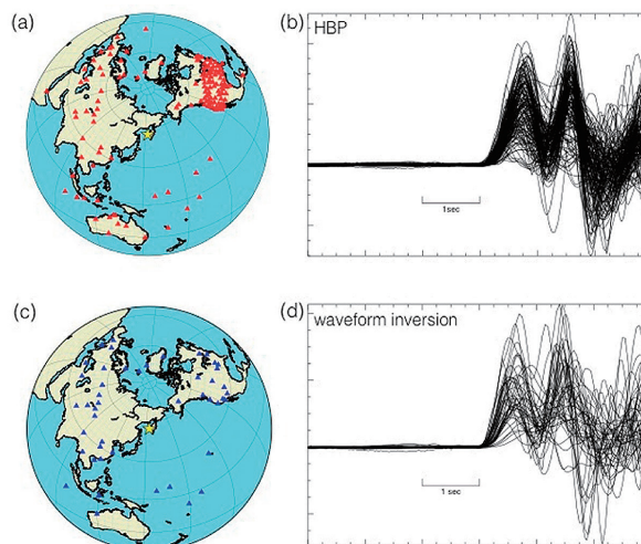
Fig. 1. Distribution of seismic stations and superposition of P waveforms. Seismic stations used for (a) hybrid back-projection (HBP) analysis and (c) waveform inversion analyses. Unfiltered vertical component P waves of the mainshock (downloaded from Data Management Center, Incorporated Research Institution for Seismology) for (b) HBP analysis at 149 stations and (d) waveform inversion analysis at 47 stations. In (b) and (d), first arrivals were picked as the first P-phase arrivals and were normalized to the maximum absolute amplitude of all waveforms. Polarity reversals were performed.
