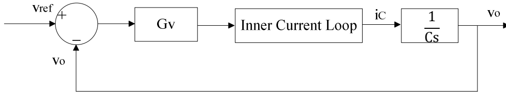
Fig. 2-6: Outer loop control diagram
