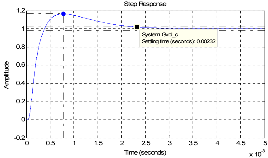
Fig. 2-8: Step response of the compensated outer voltage loop
