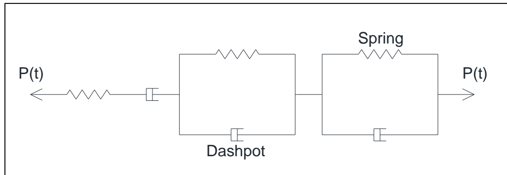
FIGURE 2 Burger's mechanical model.
