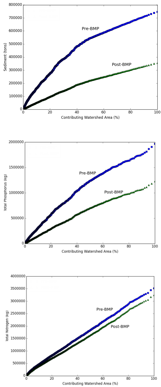
Figure 2.7. Cumulative sediment (top), total P (middle), and total N (bottom) losses by percent of contributing watershed area.
