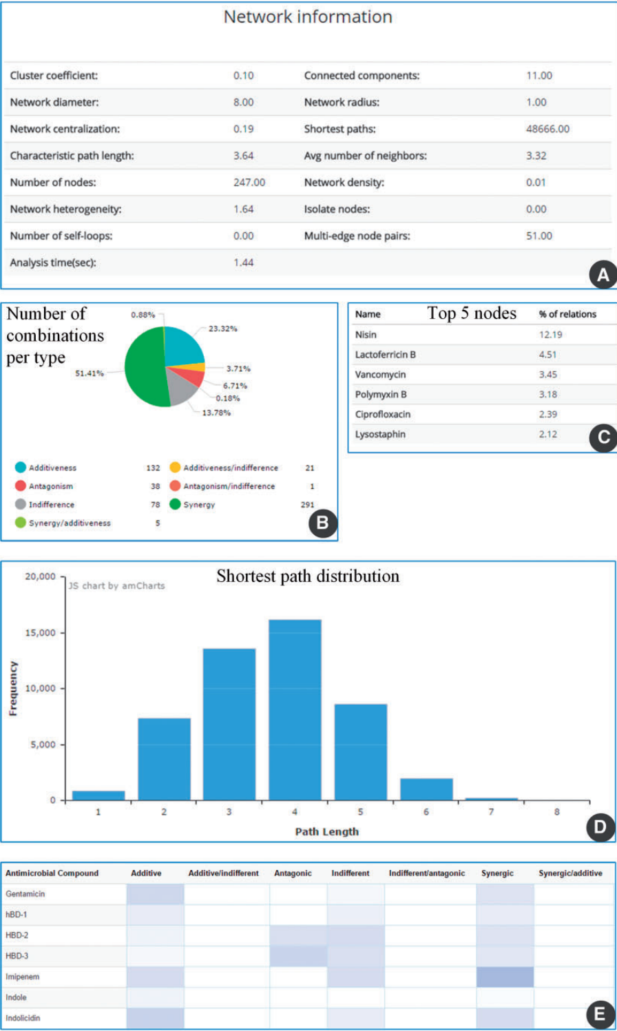
Figure 5. Details on the AMP-drug combinations tested against S. aureus . General network statistics (A) are detailed in terms of the distribution of combinations by type (B), the identification of the highest degree nodes (C), the distribution of shortest path length (D), and a snapshot of the heat map describing the distribution of all AMP-drug combinations in the database (E).
