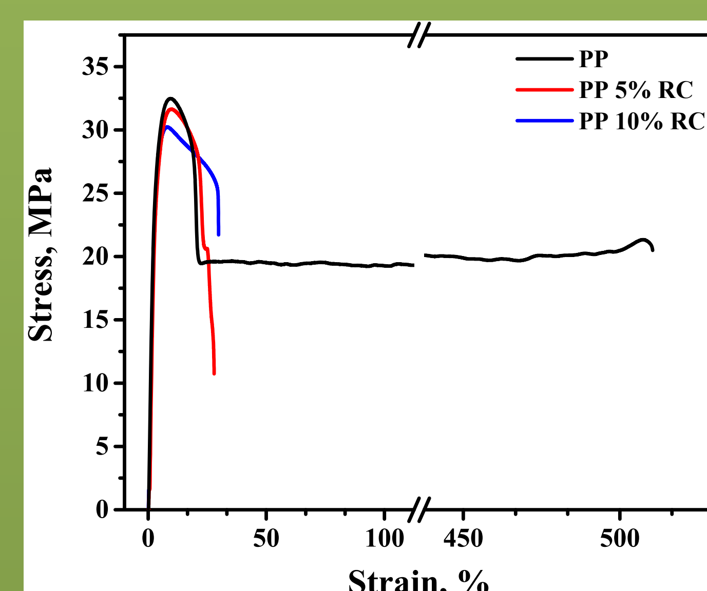
Fig. 5. Stress-strain curve of polypropylene and composite 5 % and 10% wt. residual ceramic.
