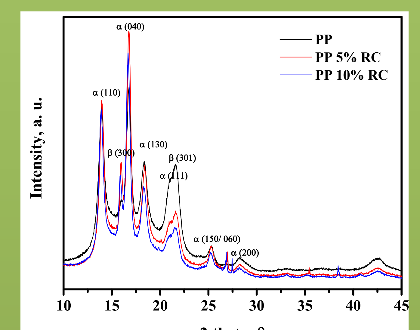
Fig. 4. XRD composite a) 5 % and 10% wt. residual ceramic.
