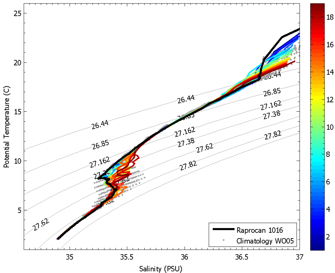
Figure 3. T-S Diagram of the sampled area.
