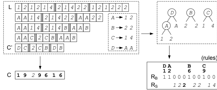
Figure 1: Example of Re-Pair compression. Solid boxes ( C and rules ) enclose the data represented. Bold numbers (nonterminals) in the final C sequence and R_S refer to positions in R_B , whereas slanted ones (terminals) refer to original values. To distinguish them, the maximum offset u is added to the bold numbers.
