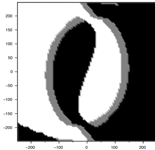
Figure 11: Optimal switching map for q = 2 for the DC/AC inverter.
