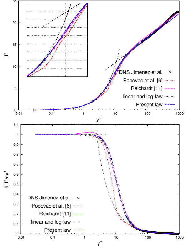
Figure 2: Comparison of the present law with that of Popovac et al.[6] and Reichardt, at Re_\tau = 950 [14]
