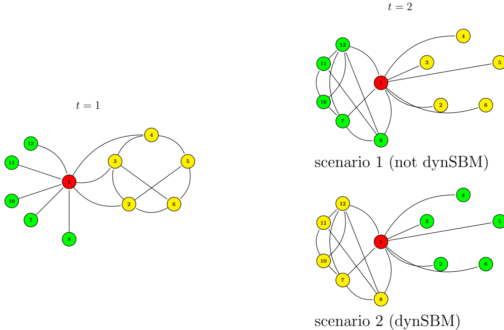
Figure 3: Adding constraints to avoid label switching between time steps. At time t = 2 there are two equivalent alternative scenarios. In scenario 1 group memberships stay constant in time and interaction parameters change with time; in scenario 2 group memberships change between the two time steps but the intra-group interactions stay constant. In this latter case, the green group is characterised by being a 'peripheral nodes' group, the yellow group is a community and the red group is a hub.
