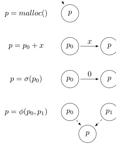
Figure 5: Rules to generate the pointer dependence digraph.
