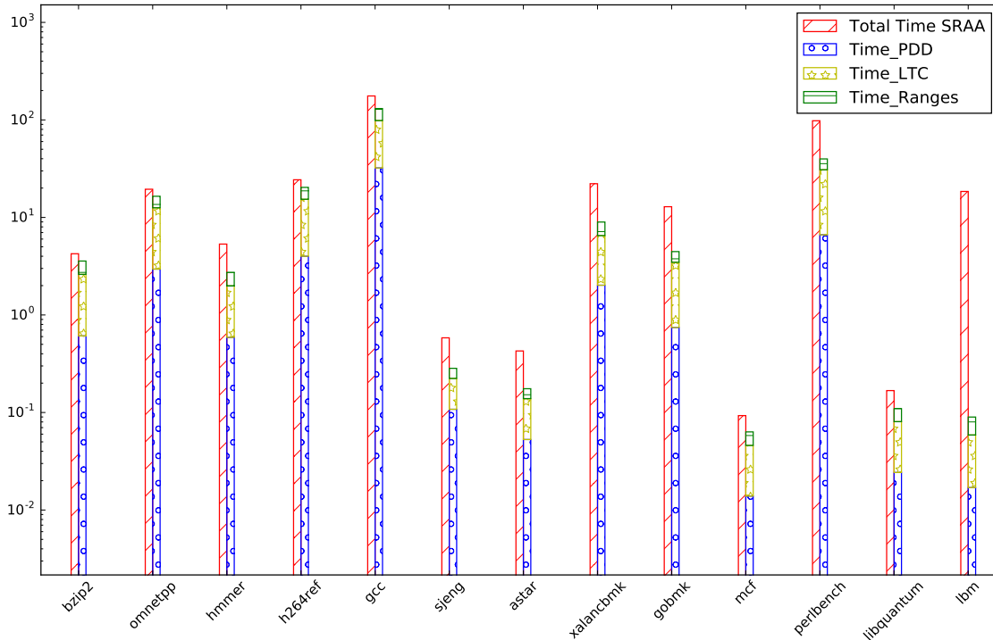
Figure 23: Time needed by each test (PDD, LTC, and Ranges) of our analysis SRAA to disambiguate SPEC-CPU2006 pairs of pointers.
