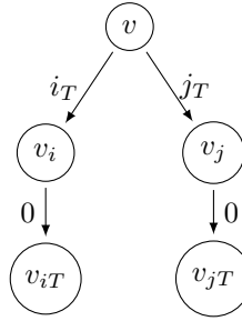
Figure 6: Pointer dependence graph of program in Figure 1a.
