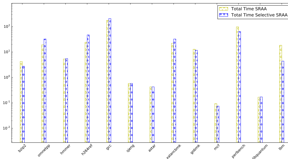
Figure 25: Comparison between time needed to run SRAA selectively (non overlapping tests) and separately (disjoint tests)
