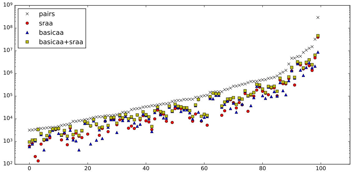
Figure 19: Effectiveness of our alias analysis (SRAA), when compared to LLVM’s basic alias analysis on the 100 largest benchmarks in the LLVM test suite (TSCV removed). Each tick in the X-axis represents one benchmark. The Y-axis represents total number of queries (one query per pair of pointers), and number of queries in which each algorithm got a “no-alias” response.
