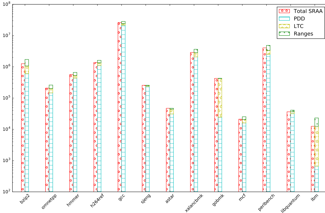
Figure 21: How three tests in SRAA separately compete to disambiguate pairs of pointers.
