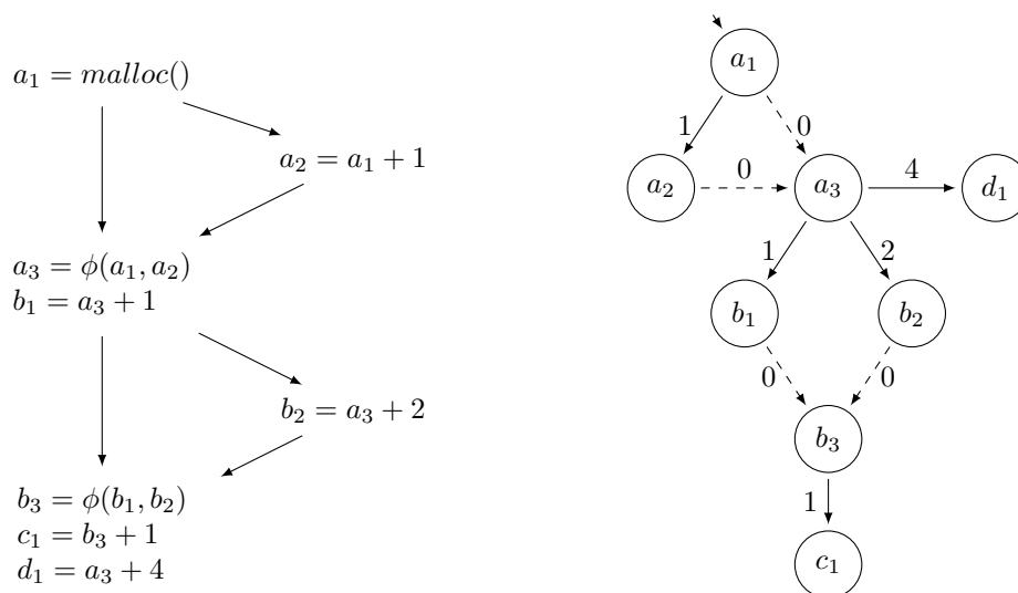
Figure 26: Illustration of the difference in precision between [[31]] and the Ranges test of this work: the program in SSA form (left) and its PDD (right)
