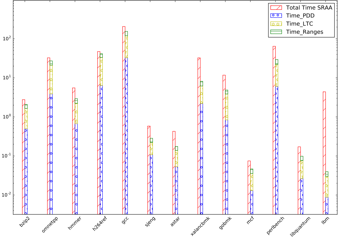
Figure 24: Time needed by each test (PDD, LTC, and Ranges) when run selectively to disambiguate SPEC-2006 pairs of pointers.
