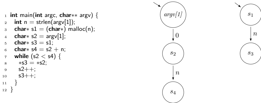
Figure 13: Program that contains two different memory locations, which will give origin to two unconnected pointer dependence digraphs. For the sake of brevity, the program is kept in high level language.
