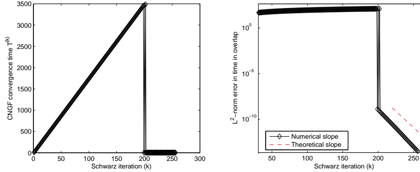
Figure 2: Two-dimensional problem with polar symmetry. Left: stopping times T^{(k)} vs. CSWR iteration k until convergence. Right: Comparison between the discrete versions of the estimated theoretical convergence rates (67) and numerical ones computed by the CSWR algorithm.
