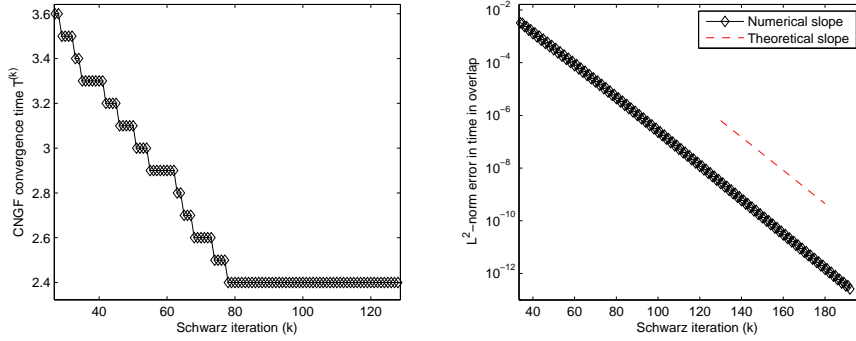
Figure 3: Two-dimensional problem with polar symmetry. Left: stopping times T^{(k)} vs. CSWR iteration k until convergence. Right: Comparison between the discrete versions of the estimated theoretical convergence rates (69) and numerical ones computed by the CSWR algorithm.
