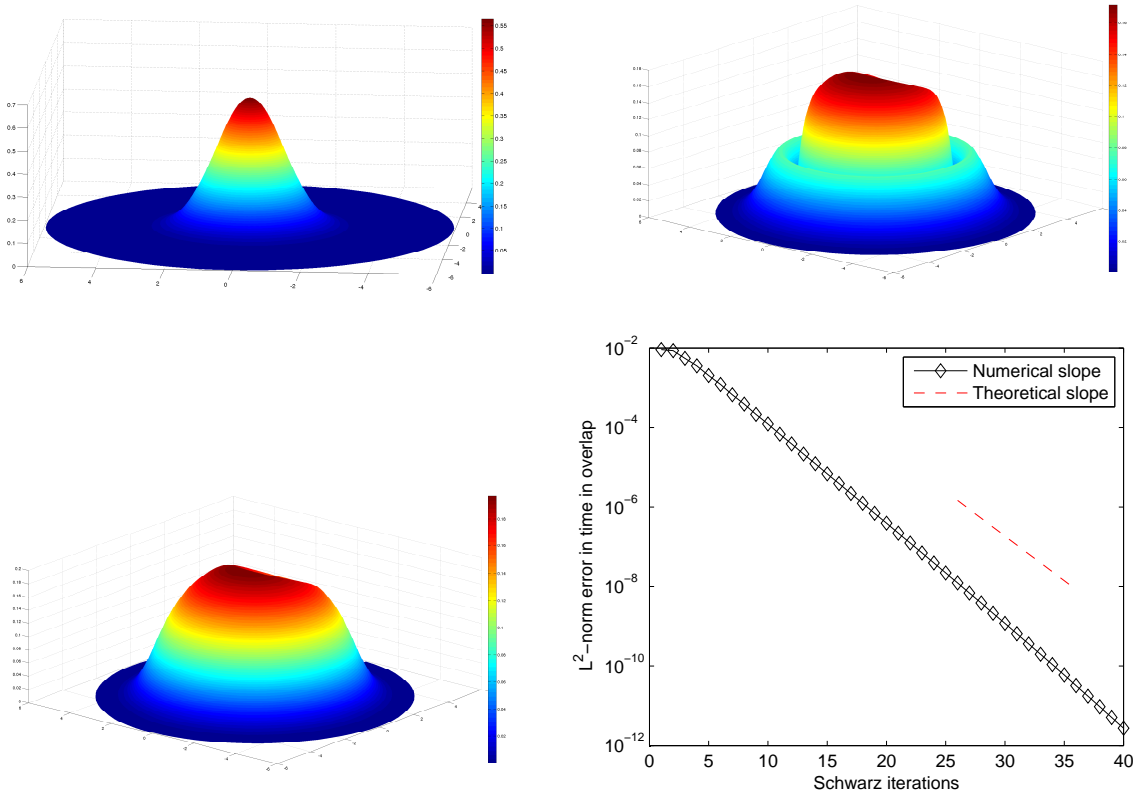
Figure 4: Two-dimensional problem without polar symmetry. (Top, left) Initial guess ( k = 0, t = 0 ), \phi_0 . (Top, right) CNGF converged solution for k = 1 , \phi^{n^{\text{CNGF}}(1)} . (Bottom, left) Converged reconstructed solution \phi^{\text{CVG}} . (Bottom, right) Comparison between the discrete versions of the estimated theoretical residual error (67), and numerical ones computed by the CSWR algorithm in a 2-d non-symmetric configuration.
