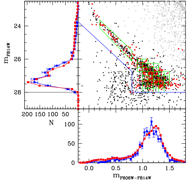
Fig. 1. White dwarf luminosity function, color-magnitude diagram, and color distribution of NGC 6397 for our best-fit model. Gray dots represent observed main-sequence stars, black dots correspond to white dwarfs, while red points denote the results of our simulations. The green squares represent the regions of the color-magnitude diagram for which we performed a \chi^2 test, while the blue thin lines correspond to the cuts adopted to compute the distributions. The red curves correspond to the simulated distributions, while the blue curves are the observed distributions computed using our cuts. See the online edition of the journal for a color version of this figure and the main text for additional details.
