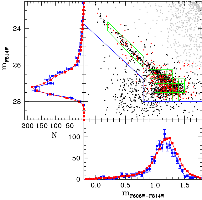
Fig. 3. Same as Fig. 1, but for the model with no residual hydrogen burning, see Sect. 4.2.
