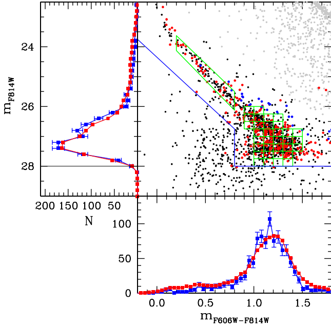
Fig. 5. Same as Fig. 1, but for a model in which we adopt a fraction of non-DA white dwarfs of 20% (see Sect. 4.4 for details).
