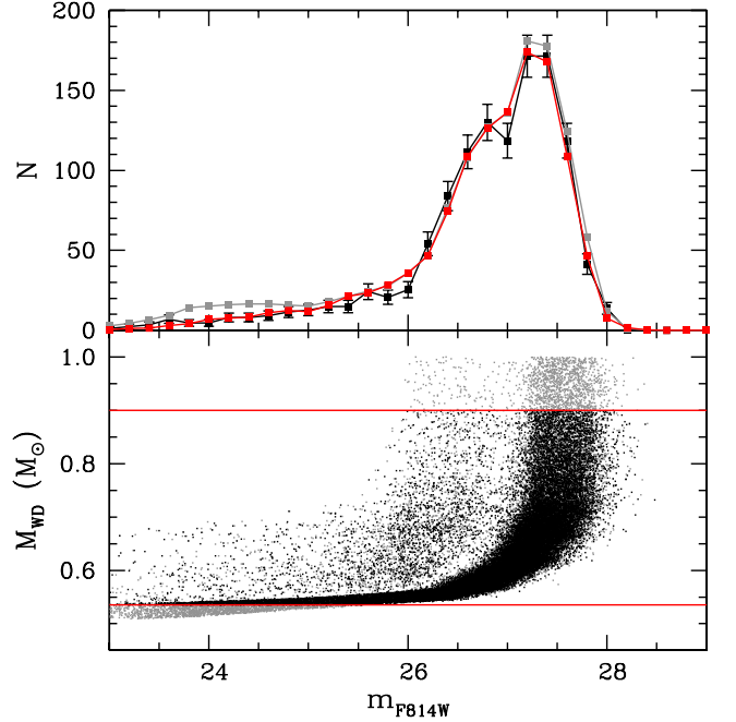
Fig. 6. Top panel: clean white dwarf luminosity function of NGC 6397 (black line) compared with the synthetic luminosity function for the entire sample of white dwarfs (gray line) and that obtained after eliminating massive and low-mass white dwarfs (red line). Bottom panel: mass distribution as a function of the magnitude for our simulated sample (black dots). The mass cuts are also displayed in this panel as horizontal red lines.
