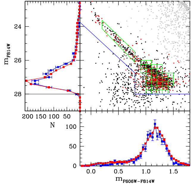
Fig. 4. Same as Fig. 1, but for the model in which the slope of the initial mass function is allowed to vary (see Sect. 4.3 for details).
