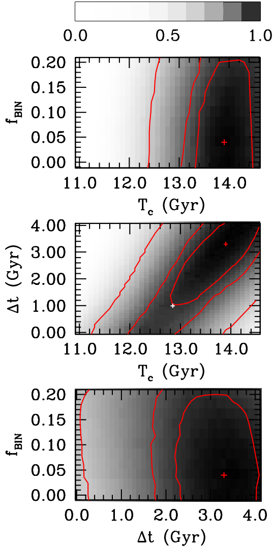
Fig. 2. Probability density distribution for different pairs of free parameters (gray scale). Marked with a cross are the best-fit values, while the red lines represent the 68%, 90%, and 95% confidence levels. The white cross corresponds to our reference model.
