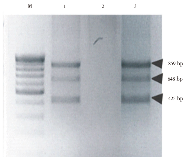
Figure 5. Amplification of mcyc sequences by multiplex PCR.
