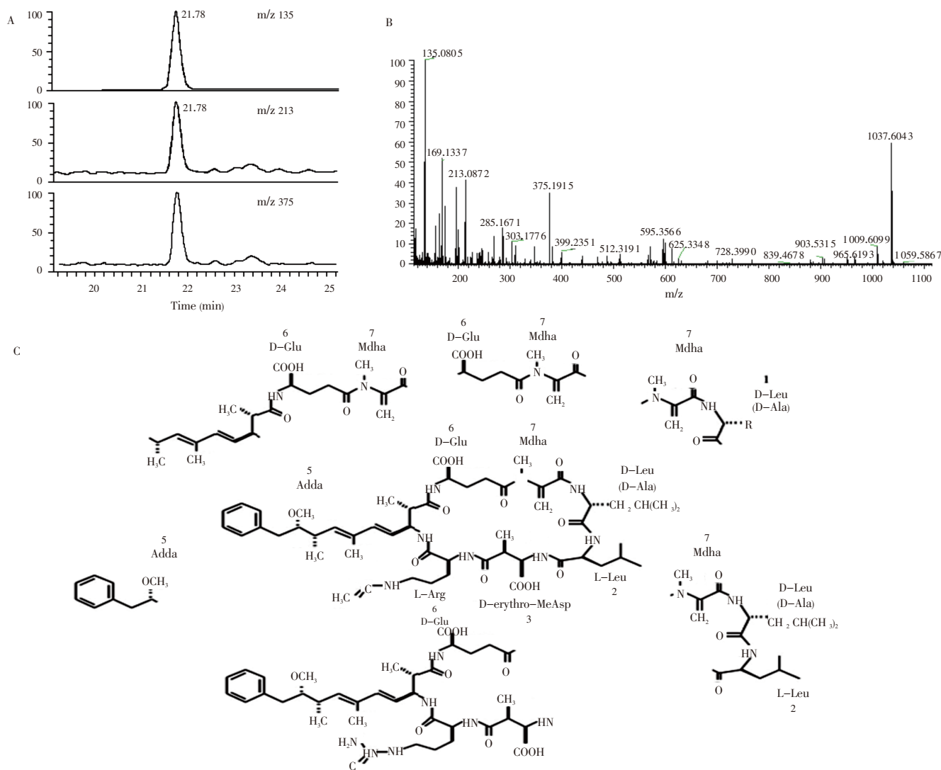
Figure 7. LC/ESI-HRMS analysis performed to confirm the identity of microcystin produced by CAAT 2005–3. A: Product ion scan data used to identify several putative metabolites for Mcyst–LRs, 135 m/z, 216 m/z and 375 m/z; B: Mass chromatogram of the [D–Leu 1 ] Mcyst–LR present in cultured samples of CAAT 2005–3 which showed the molecular ion (1037 m/z) and several metabolites; C: Fragments ions of which the [D–Leu 1 ] Mcyst–LR molecule is composed. Masp: d-erythro-b-methylaspartic acid. Adda: (2S,3S,8S,9S)–3-amino–9-methoxy–2,6,8-trimethyl–10-phenyldeca–4,6-dienoic acid. Mdha: N-methyldehydroalanine.
