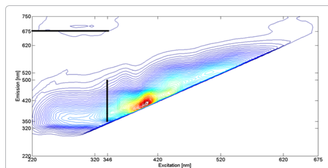
Figure 1: Selected Excitation and Emissionspectra in a 3D fluorescencespectrum of a diesel samples spiked with 0.5% EHN.
