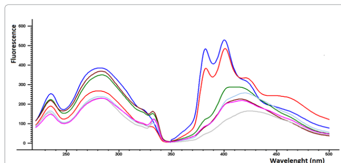
Figure 4: An EEF spectrum of the 7 commercialsamples.
