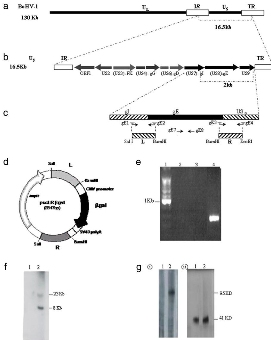
Figure 1 Molecular structure of BoHV-1ΔgEβgal virus. (a) Target region for the gE deletion in BoHV-1 genome. (b) gE ORF (US8) is flanked by gI (US7) and US9 genes. (c) Primers gE1 and gE2 were designed to amplify the left (L) fragment, and primers gE3 and gE4 were designed to amplify the right (R) fragment. The sequences of primers gE2, gE3 and gE4 were designed in order to create the depicted restriction sites to facilitate the cloning strategy. (d) pUCLRβgal recombination vector diagram restriction sites used for cloning and relative position of the elements described are shown (e) Confirmation gE-specific deletion by PCR. Lanes 2–4 primers specific to the gE sequence (gE7 and gE8) were used. Different templates were used for each lane shown: Lane 2 negative control (ultrapure sterile water); lane 3 BoHV-1ΔgEβgal DNA; lane 4 parental BoHV-1 LA DNA; lanes 1 molecular weight marker (100pb, Promega). (f) Molecular characterization of the recombinant BoHV-1ΔgEβgal strain. Southern blot analysis for gE gene. Viral DNA from BoHV-1ΔgEβgal (lane 1) and from parental BoHV-1 LA strain (lane 2) were digested with HindIII restriction enzyme, separated by 0.6% agarose gel electrophoresis, blotted to a membrane and probed with the gE probe. (g) Western blot for gE protein. Concentrated virus (BoHV-1ΔgEβgal, lane 1; and parental BoHV-1 LA, lane 2) was separated by electrophoresis in a 12% SDS-PAGE, blotted to a membrane and incubated with specific serum. Panel (i) gE-specific monoclonal antibody, panel (ii) gD-specific monoclonal antibody.
