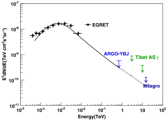
Figure 6. 99% C.L. upper limit at a median energy of 700 GeV as obtained by ARG0-YBJ for the Galactic region 130^\circ < l < 200^\circ , |b| < 5^\circ . The solid line shows the flux in the same region according to the Fermi -DGE model. The short-dashed line represents its extension following a power law with spectral index -2.6 . The EGRET results (squares) in the same region are also shown. For comparison, the upper limits from the Milagro (95% C.L., 136^\circ < l < 216^\circ , |b| < 2^\circ ) and Tibet AS \gamma (99% C.L., 140^\circ < l < 225^\circ , |b| < 2^\circ ) experiments are also reported.
