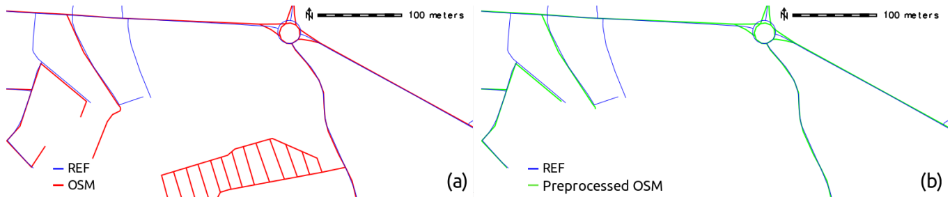
Figure 4. Example of REF and OSM datasets before (a) and after (b) the geometric preprocessing operation: OSM roads without a corresponding in the REF datasets are successfully discarded.
