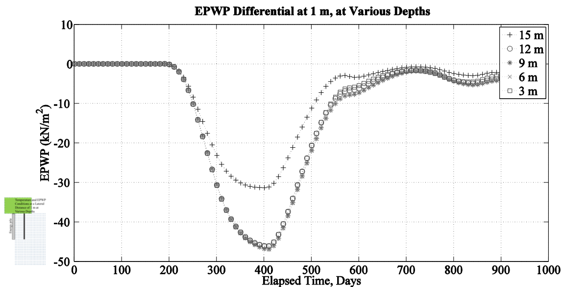
Figure 5.32. EPWP differential between model runs with and without HVAC introduction, at a lateral distance of 1 m from the pile surface at various depths. The ground-surface temperature is a constant 15^\circ\text{C} .
