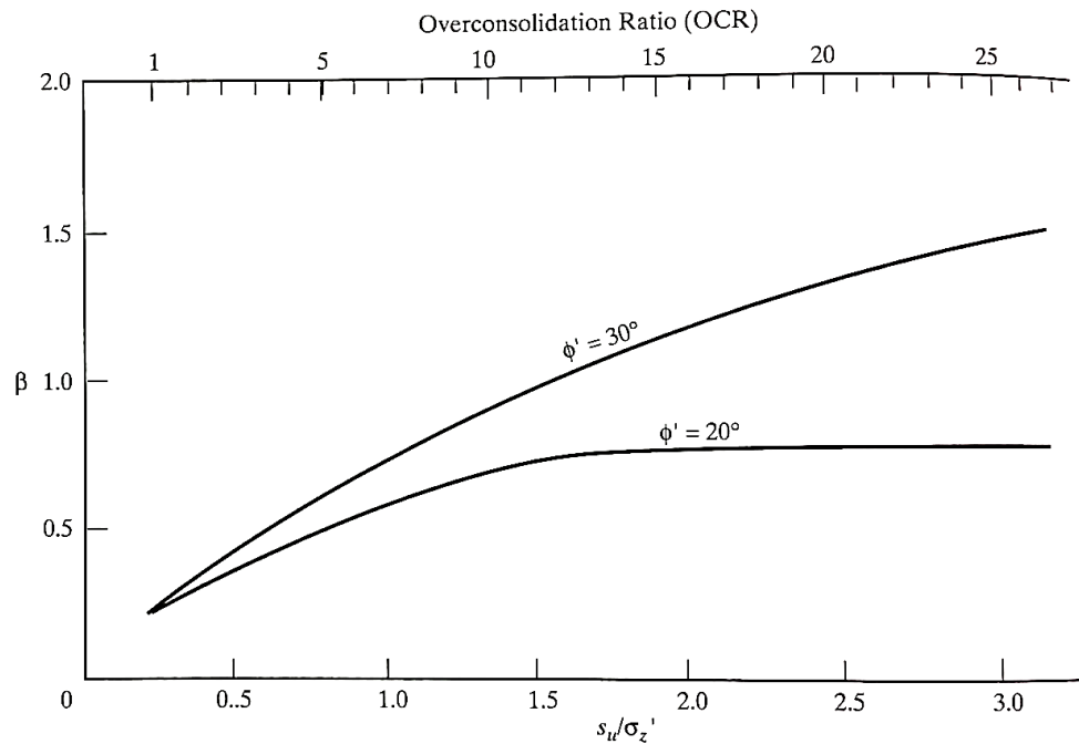
Figure 3.1. \beta value for normally to slightly over-consolidated silts and clays (Coduto, 2001) where s_u and \sigma'_z are undrained shear strength and effective vertical stress, respectively.
