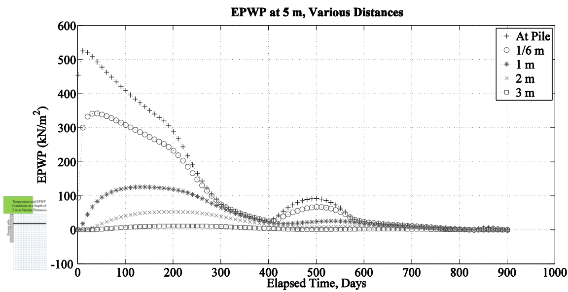
Figure C.3. EPWP at a depth of 5 m at the various distances from the pile, from the time of pile installation to the end of the model run. The ground-surface temperature is a constant 15 °C.
