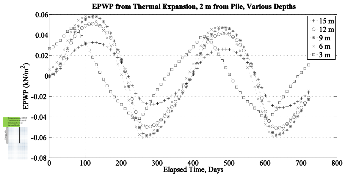
Figure 5.48. EPWP due to thermal expansion of the soil at a lateral distance of 2 m at various depths from the time of pile installation to the end of the model run, with transient ground-surface temperatures.
