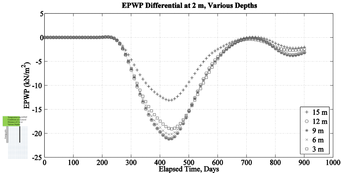
Figure 5.44. EPWP differential between model runs with and without HVAC introduction, at a lateral distance of 2 m from the pile surface at various depths, with transient ground-surface temperatures.
