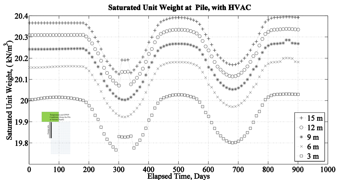
Figure 5.97. Water-saturated unit weight of soil along pile face, at various depths, with transient ground-surface temperatures and HVAC.
