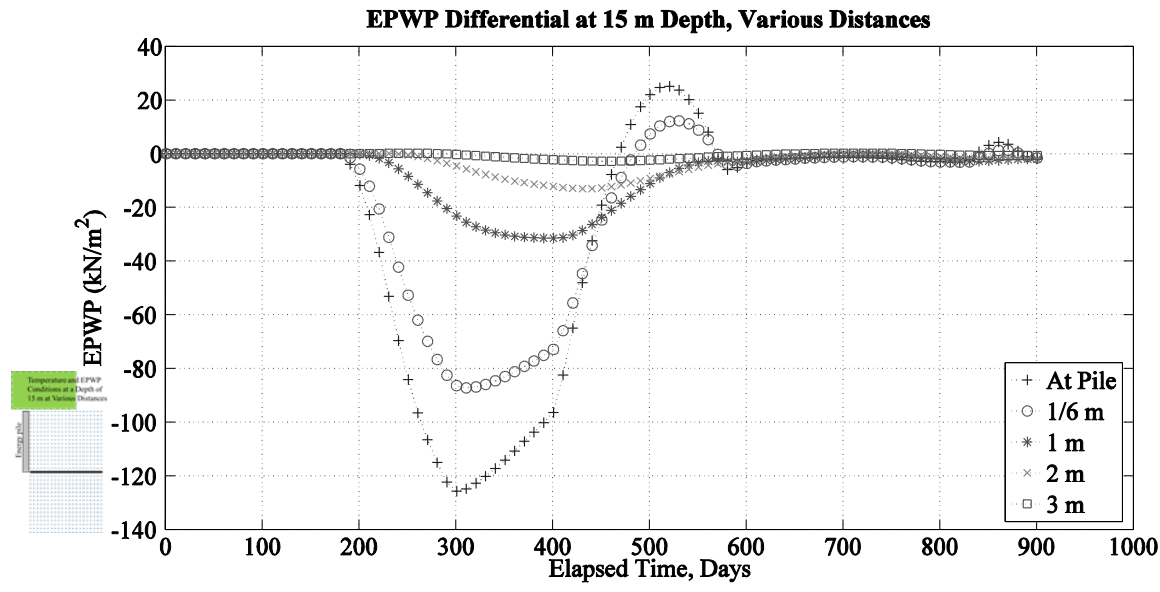
Figure C.22. EPWP differential between model runs with and without HVAC introduction, at a depth of 15 m at various lateral distances from the pile surface, with transient ground-surface temperatures.
