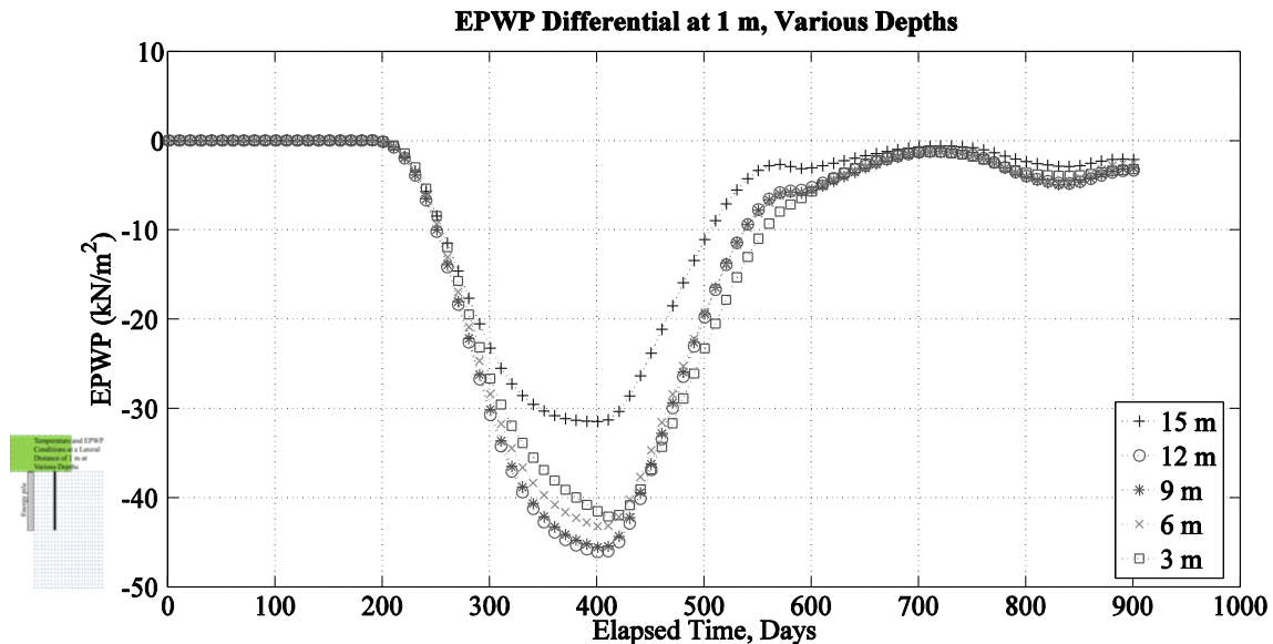
Figure 5.33. EPWP differential between model runs with and without HVAC introduction, at a lateral distance of 1 m from the pile surface at various depths, with transient ground-surface temperatures.
