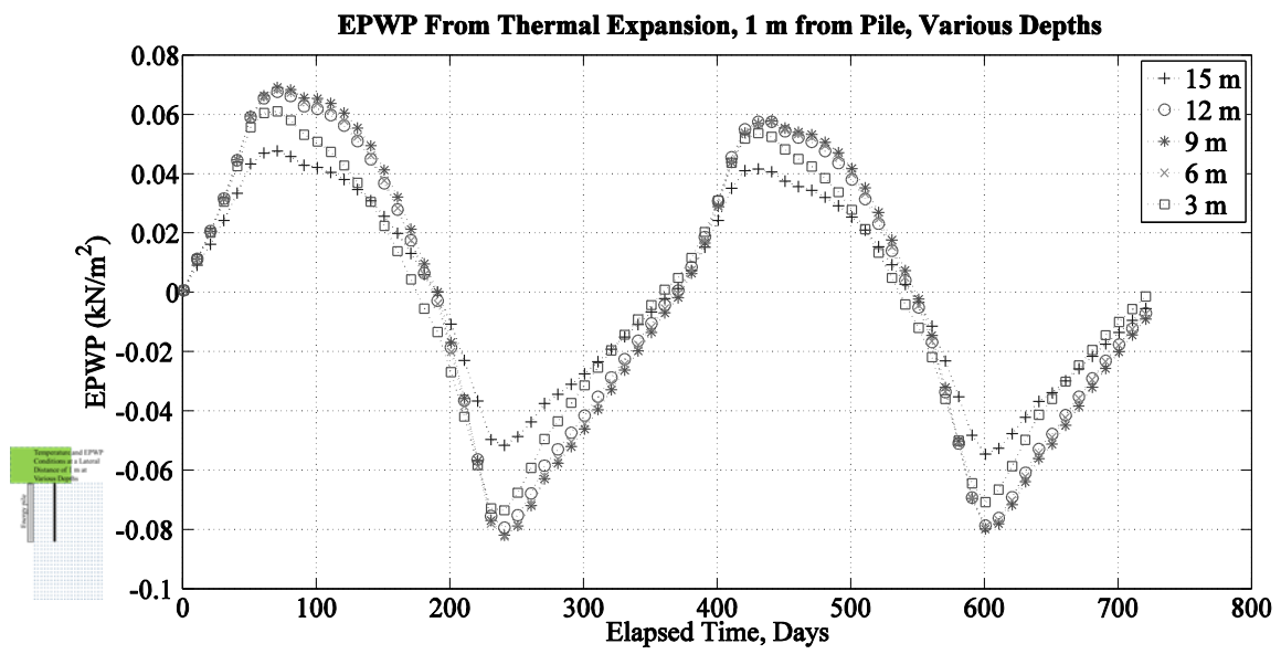
Figure 5.36. EPWP due to thermal expansion of the soil at a lateral distance of 1 m at various depths from the beginning of heating to the end of the model run. The ground-surface temperature is a constant 15 °C.
