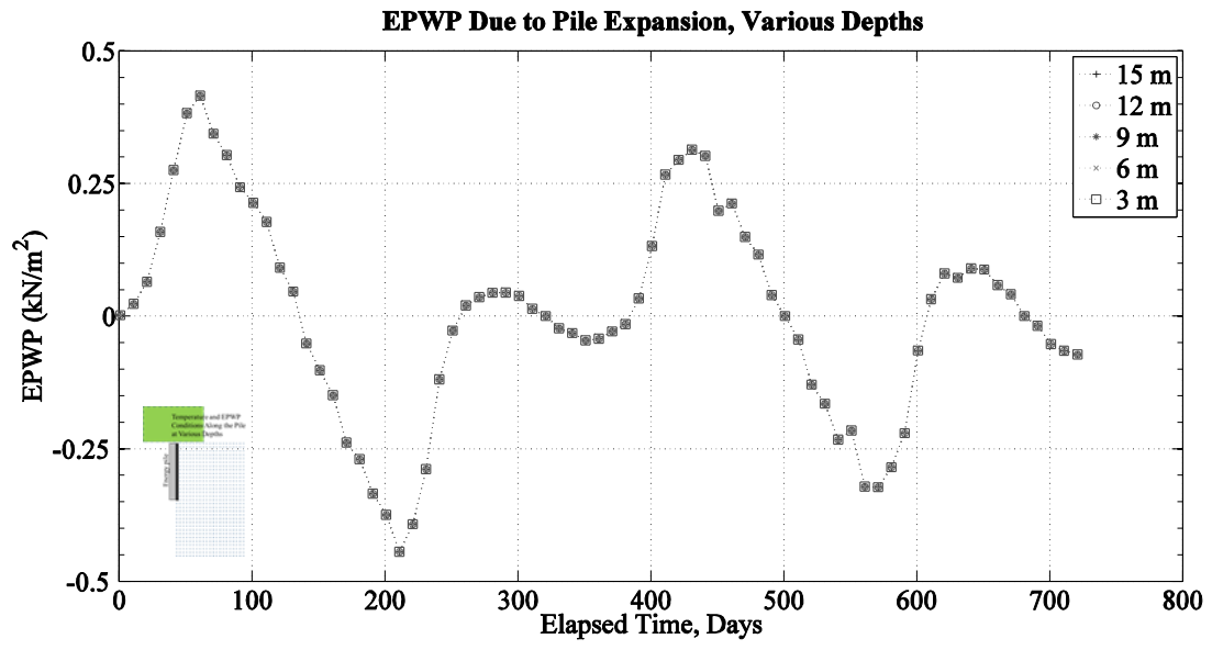
Figure 5.12. EPWP due to thermal expansion of the pile along the pile surface at various depths from the beginning of heating to the end of the model run. The ground-surface temperature is a constant 15 °C.
