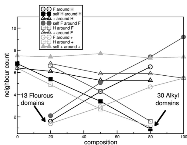
Figure 6. Neighbor count from Table 2 plotted against the composition of [\text{C}_8\text{C}_1\text{Im}][\text{Br}] mixed with [(\text{C}_p)_6\text{C}_2\text{C}_1\text{Im}][\text{Br}] . F: “Fluorous”; H: “alkyl”, +: “ring” moieties. Black: neighbor count around “alkyl”, dark gray: neighbor count around “fluorous”, light gray: neighbor count around polar “ring” groups.
