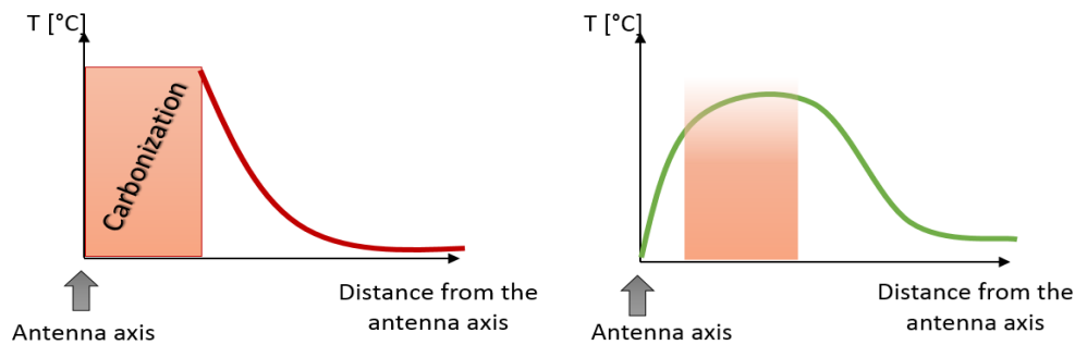
Figure 3.2.4 Sketch of the presumible thermal profile occurring in the MTA treated tissue radially to the antenna feed. Left: in presence of carbonization (HS and MS cases); right: in absence of carbonization (CV case < 5 min).
