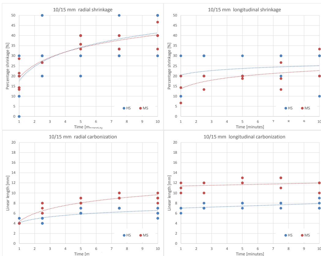
Figure 3.1.11 Percent tissue shrinkage (top) and absolute dimension of carbonization (bottom) as a function of time obtained at the end of the ablation procedure in cubes smaller than 20 mm side for two different ablating systems: Acculis™ MTA System AngioDynamics (MS), and Amica™ system HS Hospital Service SpA (HS). Left: radial; right: longitudinal.
