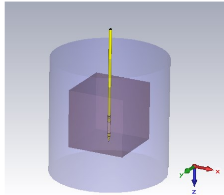
Figure 3.4.10 Design of a MTA antenna (yellow) in a cube of liver tissue (light purple brick) embedded in an Agar phantom (light blue cylinder), with Cartesian coordinates (CST software).
