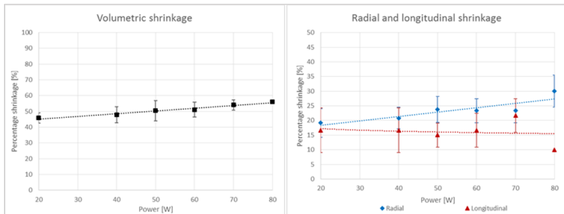
Figure 3.1.6 Percent tissue shrinkage obtained as a function of power ablating 20 mm side cubes with the MiW Amica™ system, HS Hospital Service SpA (HS), for 5 min; left: volumetric shrinkage; right: radial and longitudinal shrinkage.
