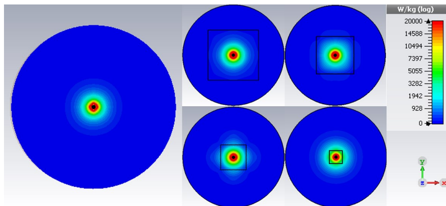
Figure 3.4.11 SAR map into the tissue surrounding the MTA antenna; xy -plane orthogonal to the antenna axis in correspondence to the antenna feed; unrestricted liver tissue (left) and cubes of liver tissue of different sizes (black wire boxes from top left to bottom right: 40 mm, 30 mm, 20 mm, and 10 mm side) embedded in agar phantom.
