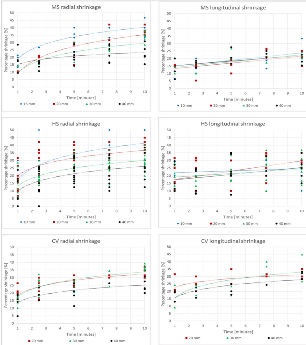
Figure 3.1.8 Percent tissue shrinkage obtained from microwave ablation as a function of time for different cubes' size and devices. From top: Acculis™ MTA System AngioDynamics (MS), Amica™ system HS Hospital Service SpA (HS), and Emprint™ Covidien (CV). Left: radial; right: longitudinal.
