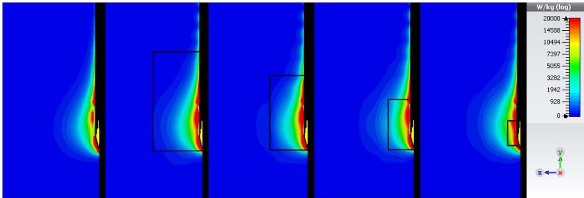
Figure 3.4.12 SAR map into the tissue surrounding the MTA antenna; yz -plane parallel to the antenna axis; unrestricted liver tissue (left) and cubes of liver tissue of different sizes (black wire boxes from left to right: 40 mm, 30 mm, 20 mm, and 10 mm side) embedded in agar phantom.
