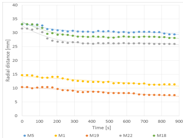
Figure 3.3.5 Radial markers' trends as a function of time: markers moving toward the antenna axis.
