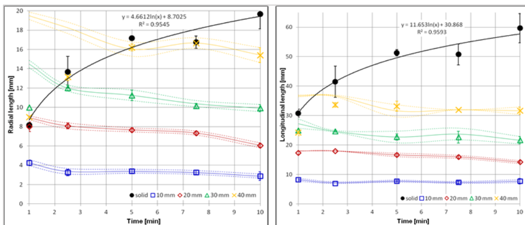
Figure 3.1.5 Comparison between the extension of the coagulated area and the post-ablation cubes' dimension; dots: carbonized area, lines: cubes' post-ablation dimension. Black line: interpolation of the unrestricted tissue data.
