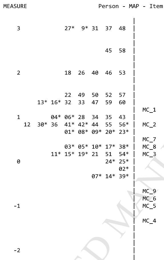
Wright map
