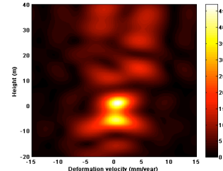
Fig. 3 Single-look adaptive Diff-Tomo output (amplitude) for a sub-Rayleigh double scatterer, real ERS-1/2 satellite data
