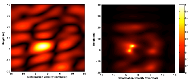
Fig. 2 Diff-Tomo output (normalized amplitude) for a sub-Rayleigh double scatterer, simulated data, left: single-look Fourier, right: single-look adaptive (same colorbar for both)
