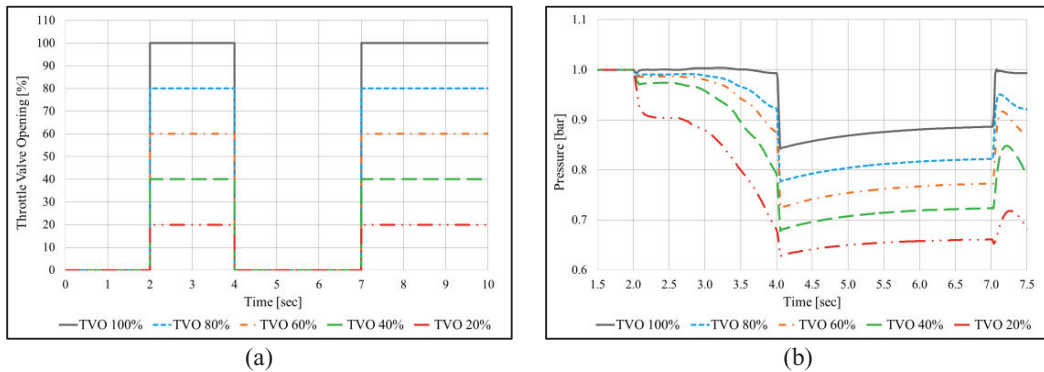
Fig. 8. (a) Throttle valve opening (TVO) profiles (%) imposed in the engine-vehicle model for transient simulation.
