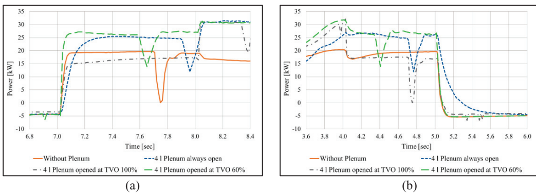
Fig. 13. Engine power during transient numerical analysis. Comparison among engines equipped with different intake systems (without the plenum, with the plenum always open, with the plenum opened only when WOT condition is reached and with the plenum opened only when 60% of the maximum TVO is reached).
