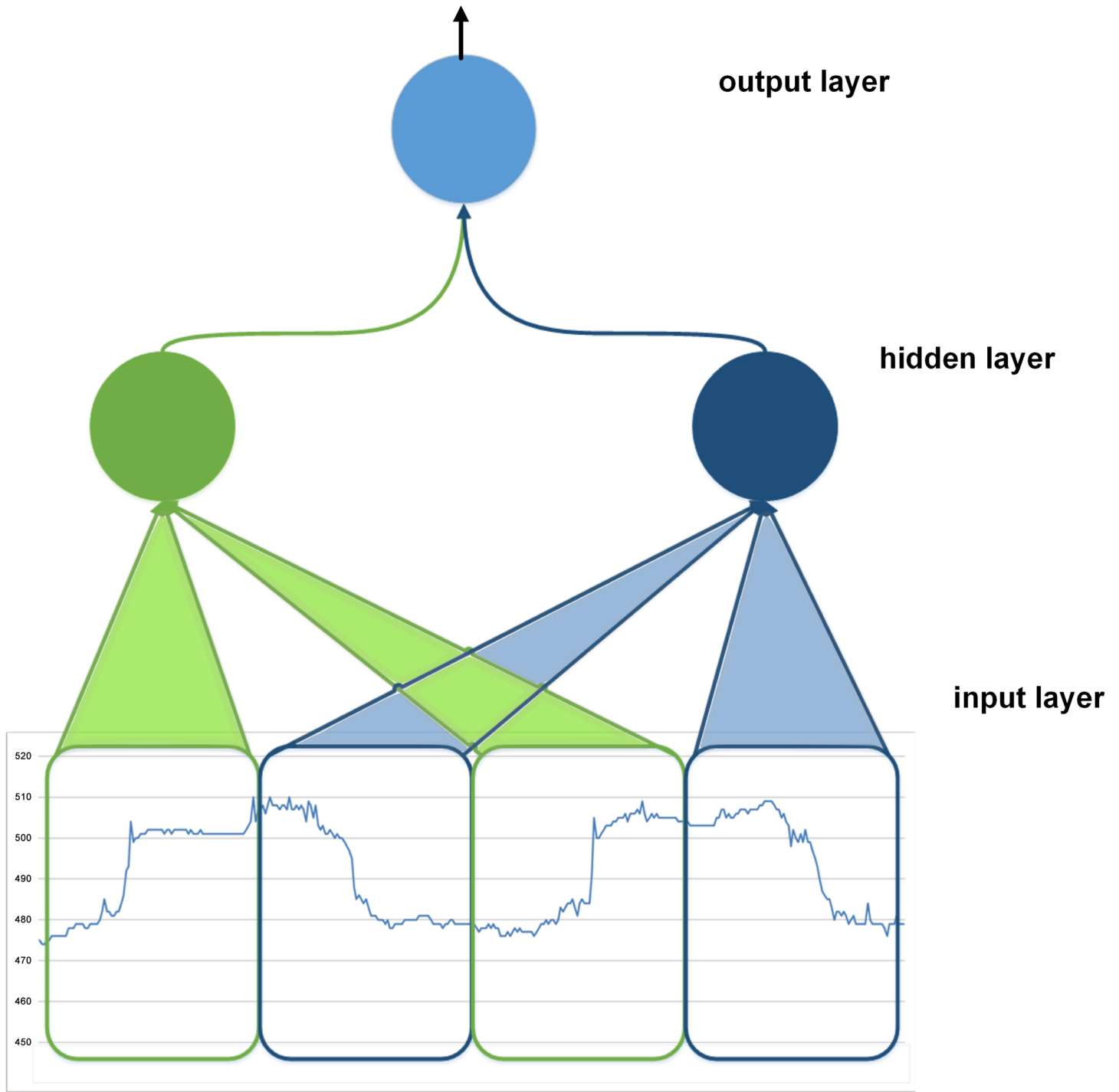
Fig 9. Input delay neural network with LRF and weight sharing (IDNN LRF WS). The input window relates the four sub-windows identified for IDNN LRF. With characteristic pattern divided in sub-windows, both the first and the third sub-windows are in an ascent phase of the squared signal, whilst the second and the fourth sub-windows are in the descent phase. The colours of the connections highlight the sharing of weights between hidden units due to the match between sub-windows. Weights are shared between the two sub-windows that make up each phase: i.e. each unit uses the same set of weights for both the sub-windows of the ascending and descending phase (we identify this model as IDNN LRF WS).
