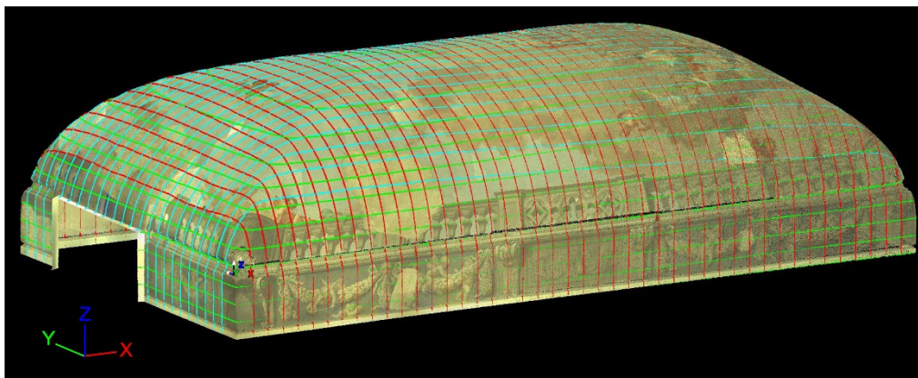
Figure 2. Dense contour model (isometric view).
