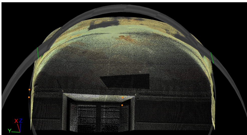
Figure 4. Approximation by cylindrical surface.
