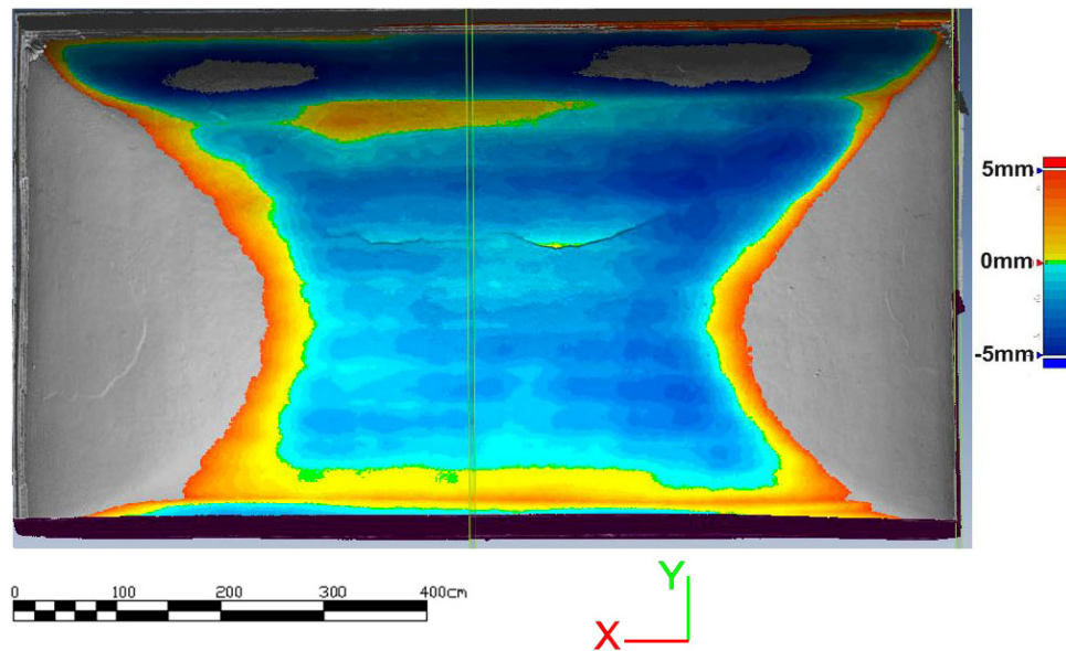
Figure 5. Actual 3D model—Cylindrical surface error.
