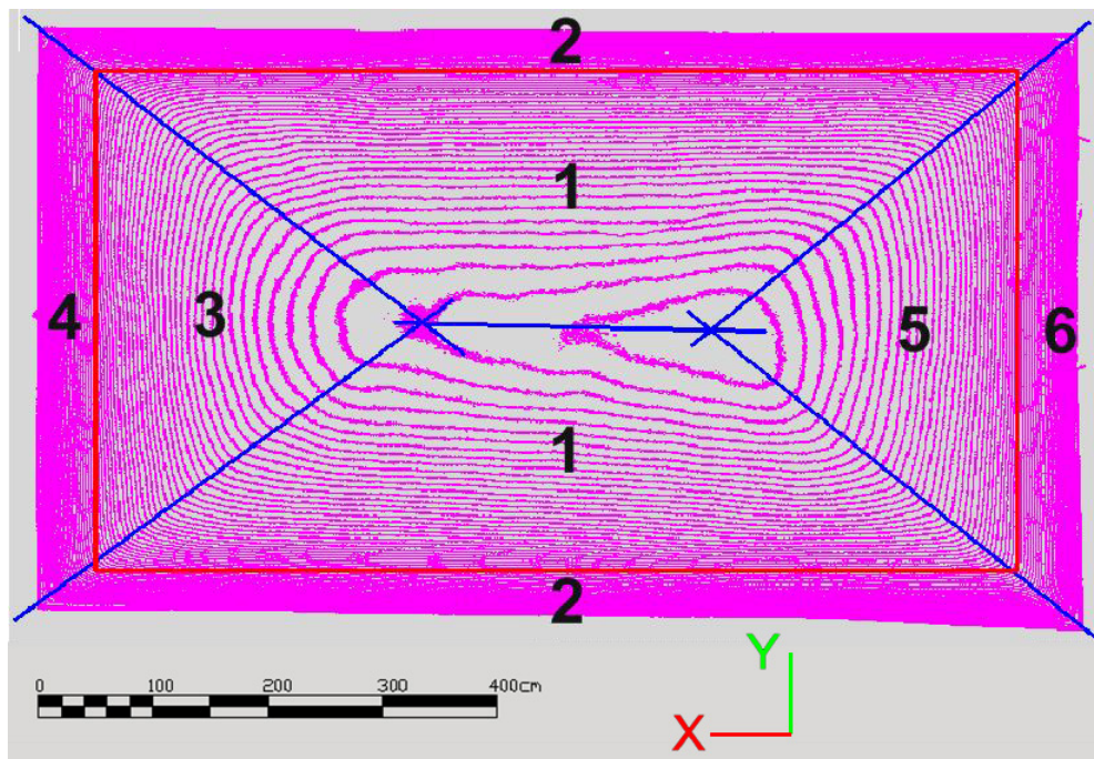
Figure 3. Discontinuity directions and vault areas (bottom view).
